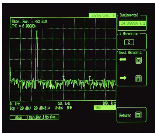
Harmonic distortion
